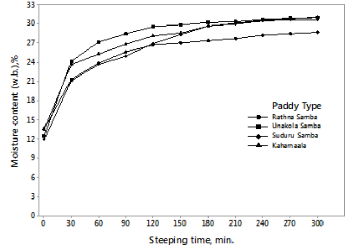
Figure 1. Moisture absorption capacities of Rathna samba , Unakola samba , Suduru samba and Kahamaala at 70 °C
